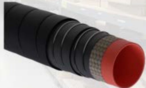
8" X 33FT ALFAGOMMA BOOM HOSE
